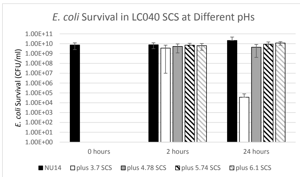
Figure 6: E. coli survival in buffered SCS from LC040. The buffer used is \text{KH}_2\text{PO}_4/\text{K}_2\text{HPO}_4 . The untampered SCS had a pH of around 3.7. The buffered SCSs had pHs of 4.78, 5.74, and 6.1.
